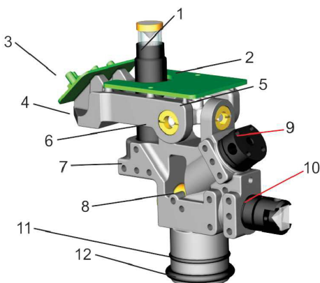
1.1 Pendulum Structure
